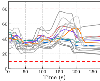
Decentralized HK-RPC
