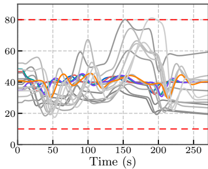
Single-CAV MPC
