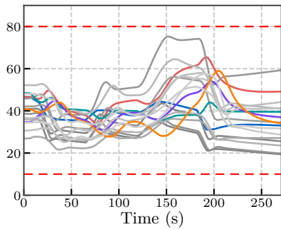
Distributed HK-RPC
