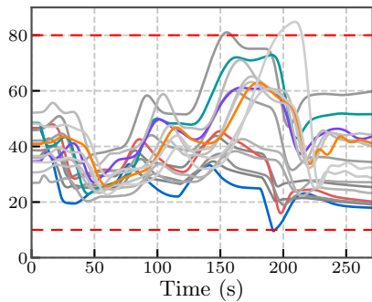
Distributed DeePC
